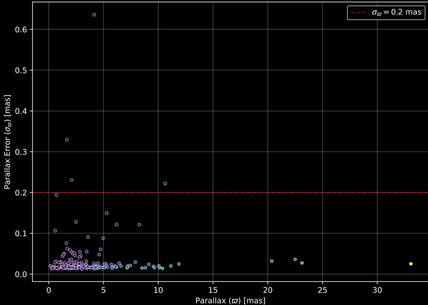
APOGEE DR17 Field: [176-49_MGA] Parallax Quality (n= 201)
