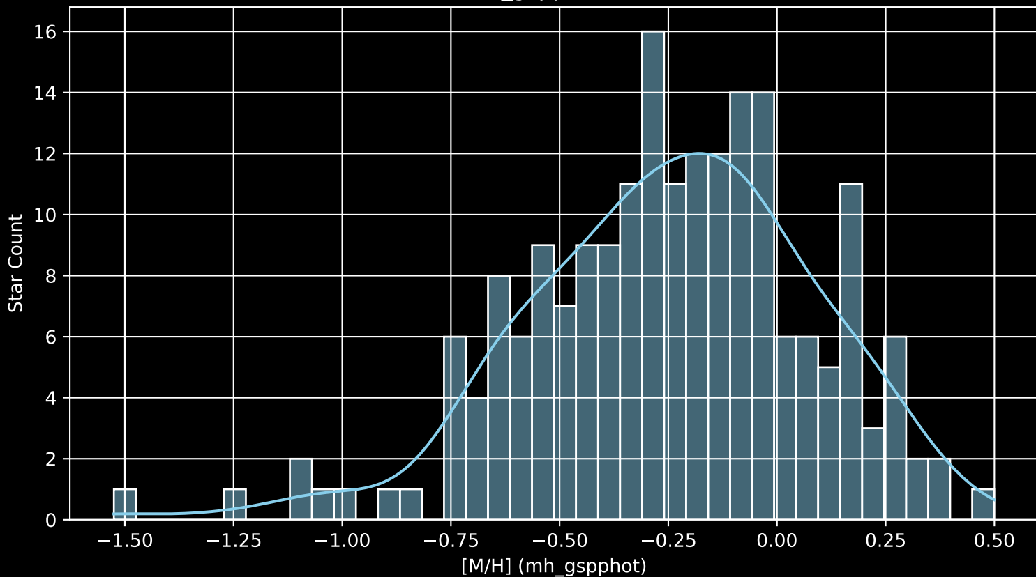
APOGEE DR17 Field: [176-49_MGA [M/H] (mh_gspphot) (n= 198)
