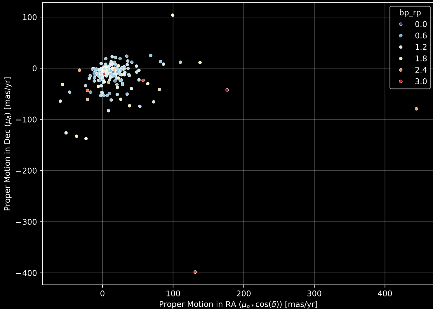
APOGEE DR17 Field: [176-49_MGA] Proper Motion Diagram (n= 201)
