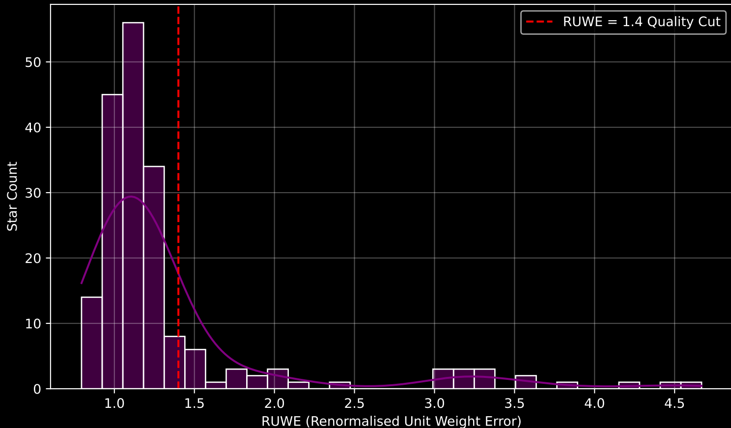
GAPOGEE DR17 Field [176-49_MGA] RUWE Distribution (n= 189)
