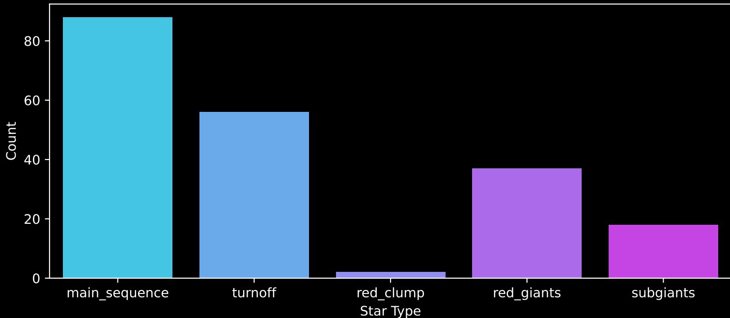
APOGEE DR17 Field: [176-49_MGA] Count plot of Star Type
