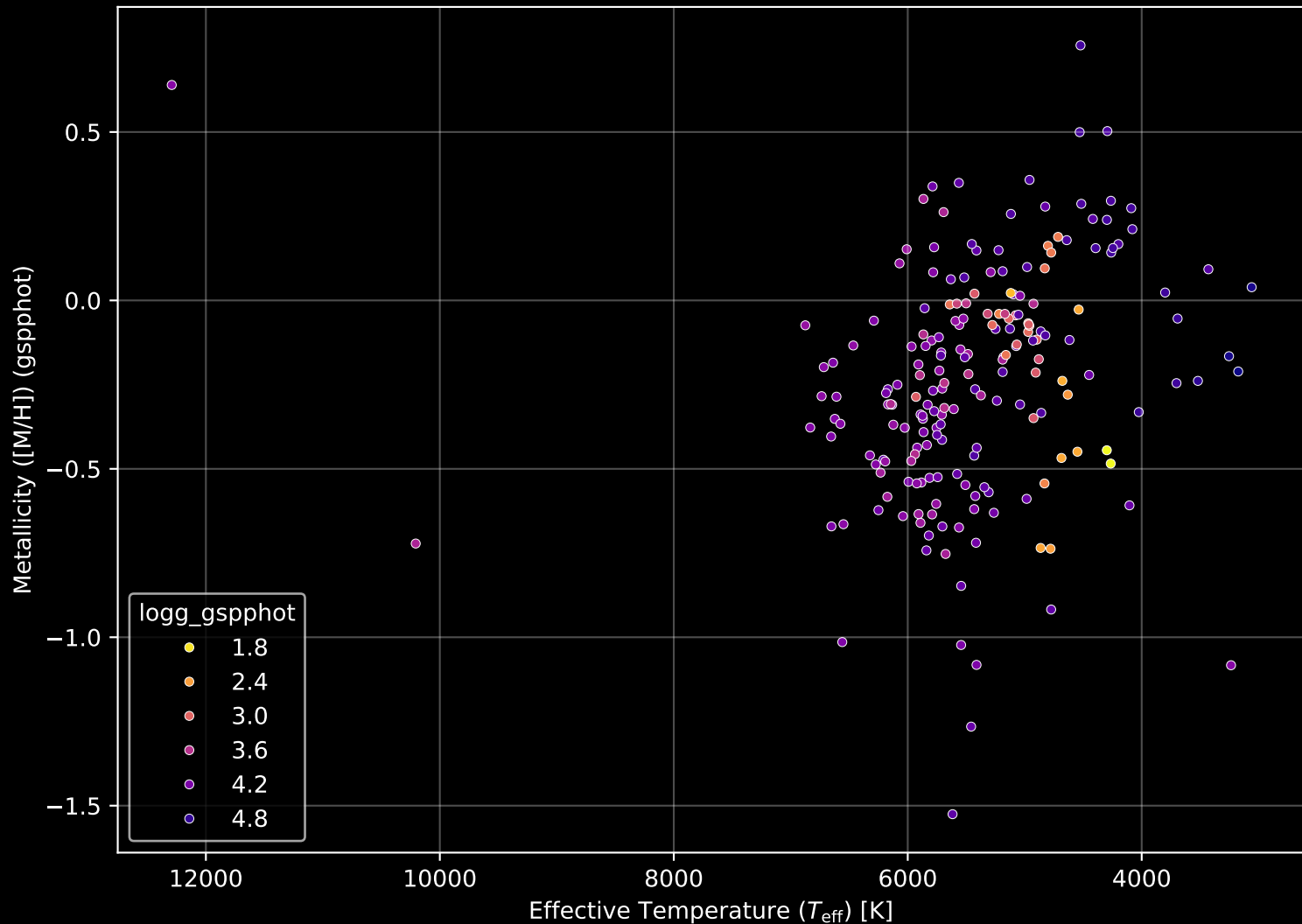
APOGEE DR17 Field: [176-49_MGA] Stellar Population Parameters (n= 201)
