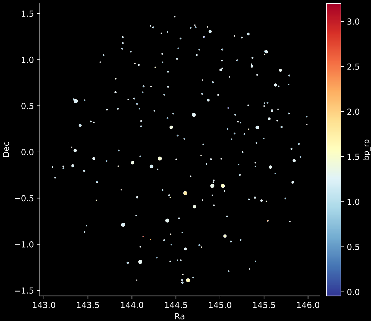
APOGEE DR17 Field: [176-49_MGA] Stars: 201
